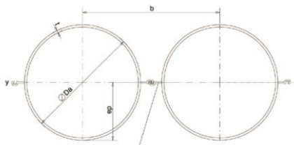
Steelwall connectors LPB 180-12
